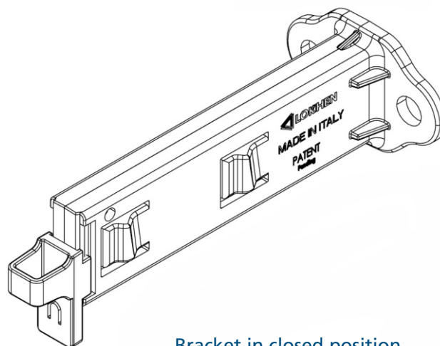
Bracket in closed position
