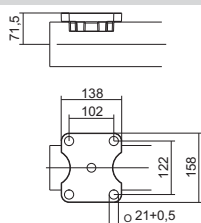
Widok "X"
